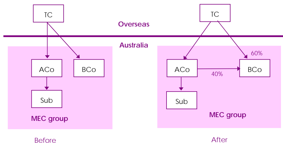
Figure 3: CGT event
